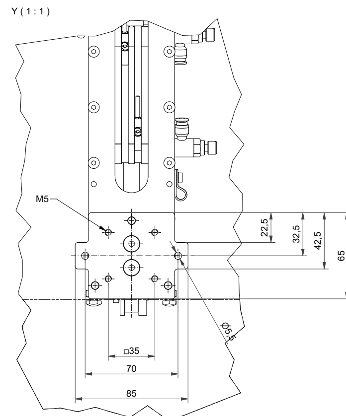
Dimensions of the connective plate (for gripper)
